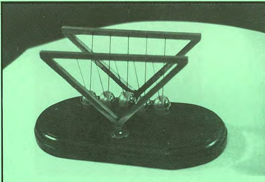
Newton's Cradle 5th Form Workshop Technology Project by M Fracklin
